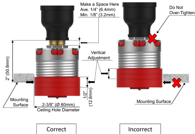
Figure 3: Installation
