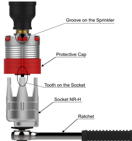
Figure 4: Ratchet & Socket
